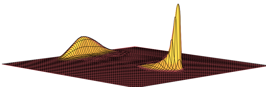
ONE-HALF REVIVAL of a wave packet ( left )—that is, the formation of two smaller packets after the original has dispersed—takes place after about 15 orbits. It is indicated by
